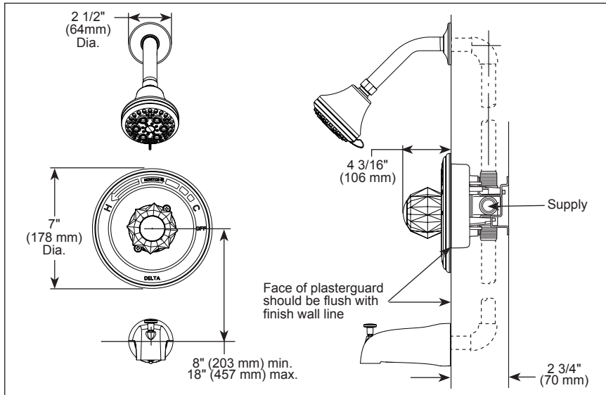
RP101727▲ Pull-Up Diverter
